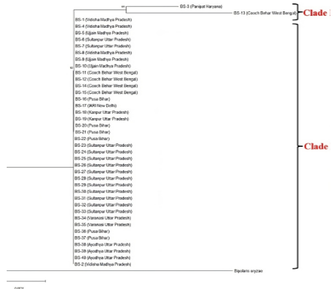
Fig. 1. Phylogenetic tree of ITS sequences in 40 B. sorokiniana
