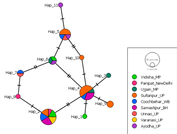
Fig. 6. Haplotype analysis for concatenated sequences of SCD1 and BRN1 virulence genes
